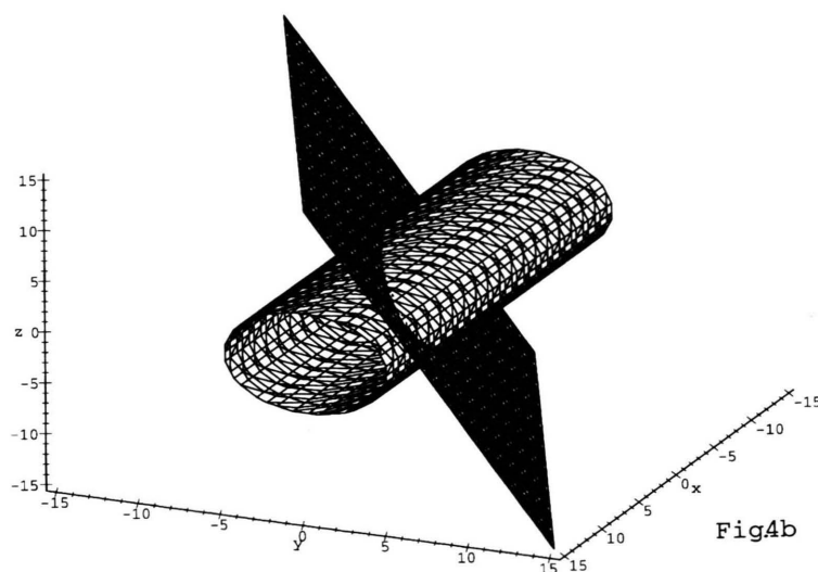
Fig. 4. (a) An equi-potential plot of a single (3+1)-dimensional ring soliton solution at time t = 0 for the potential ux \equiv -u_x = 0.0005 with the condition (39) and r_{011} = 5 . (b) The plan x - 2y - z = 0 and the cylinder y^2 + z^2 - 25 = 0 related to the ring soliton solution shown by Fig. 4a.
