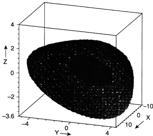
Fig. 3. An equi-potential plot of a single (3+1)-dimensional dromion solution for the potential ux \equiv -u_x with the condition (39) at time t = 0 . The inner small equi-potential shell is related to ux = 0.1 and the outside large equi-potential shell is related to ux = 0.0001 .
