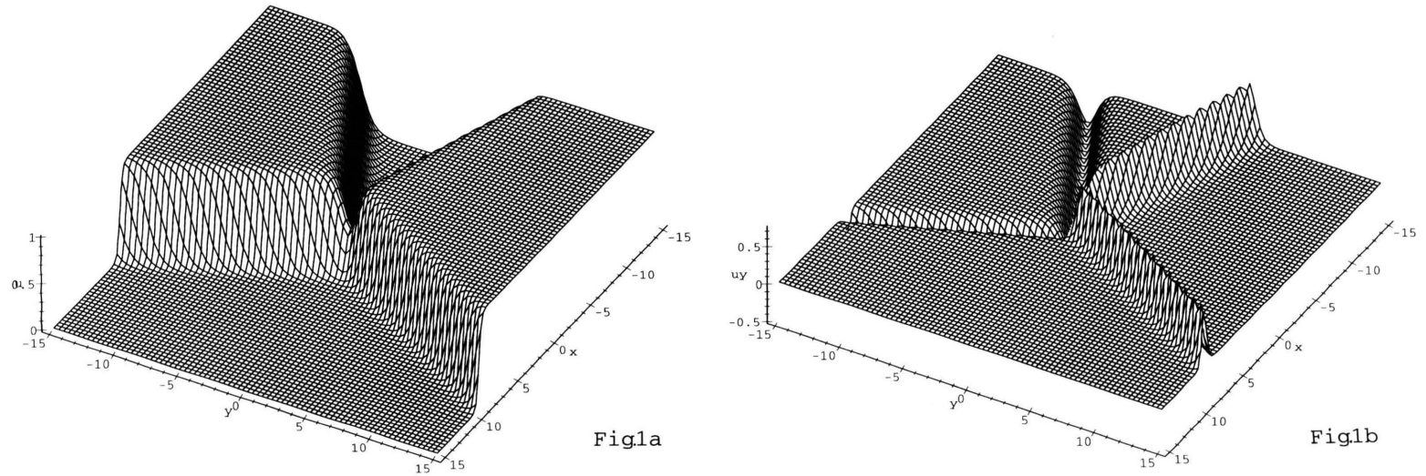
Fig. 1. Three types of multiple line soliton solutions. (a) A four straight-line soliton solution (31) in 2+1 dimensions at time t = 0 for the field u with conditions (34) and n = 1 , y_1 = y , while f is given by (33). (b) A plot of the four straight-line soliton solution with the same condition as Fig. 1a for the potential u_y \equiv uy . (c) A plot of another type of line soliton solution in 2+1 dimensions for the field u with n = 1 , y_1 = y . f is given by (33) with the conditions (35) at time t = 0 .
