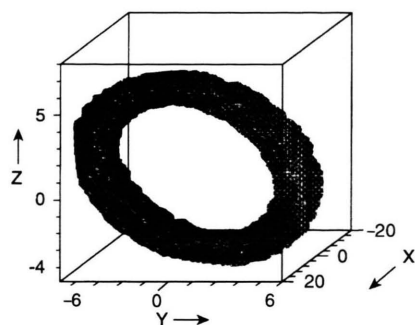
Fig. 4. (a) An equi-potential plot of a single (3+1)-dimensional ring soliton solution at time t = 0 for the potential ux \equiv -u_x = 0.0005 with the condition (39) and r_{011} = 5 . (b) The plan x - 2y - z = 0 and the cylinder y^2 + z^2 - 25 = 0 related to the ring soliton solution shown by Fig. 4a.
